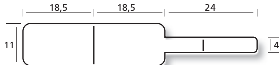
44 1161 B = 1, BB = 88 mm, T = 3/6"
