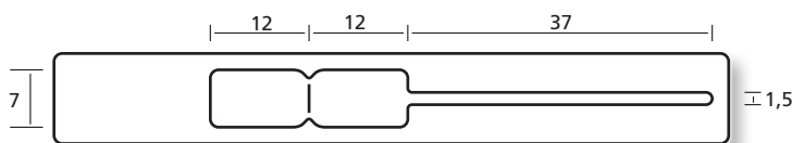
34 761/1IR B = 1, BB = 90 mm
