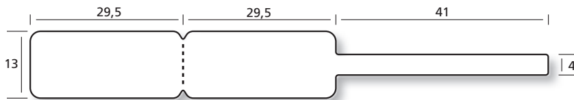
44 13100 B = 1, BB = 130 mm, T = 4/6" EAN-13
