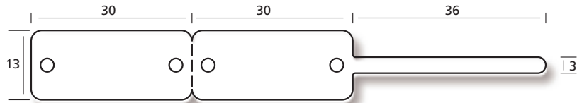
34 1396L B = 1, BB = 110 mm
