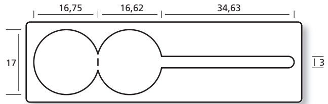
34 1768/2IR B = 1, BB = 80 mm
