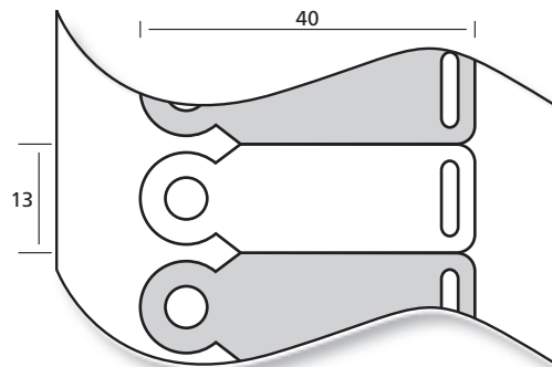
35 1340* B = 1, BB = 40 mm
