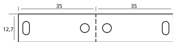
45 1270/3* B = 1, BB = 120 mm, T = 3/6"
