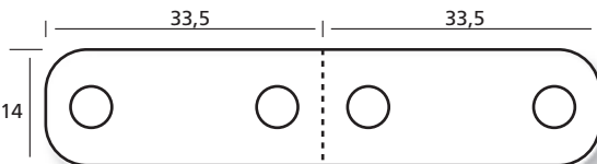
45 1467 B = 1, BB = 100 mm, T = 4/6"
